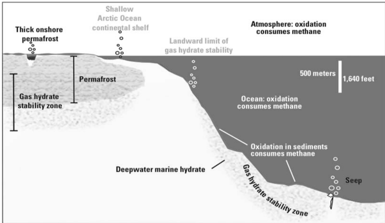
Schematic cross section showing gas hydrate within and beneath permafrost (left side) and in deepwater marine sediments (right side). The locations described in orange are the most susceptible to climate processes that can affect the stability of methane hydrate deposits. Oxidation shown in red can destroy methane in sediments, in the water column, and in the atmosphere.
